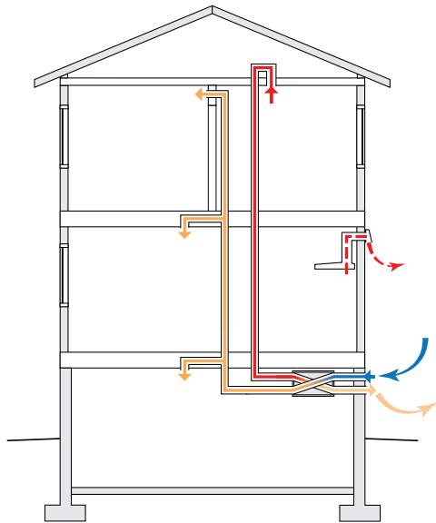
Figure 3.20 Schematic layout of a standalone HRV system
